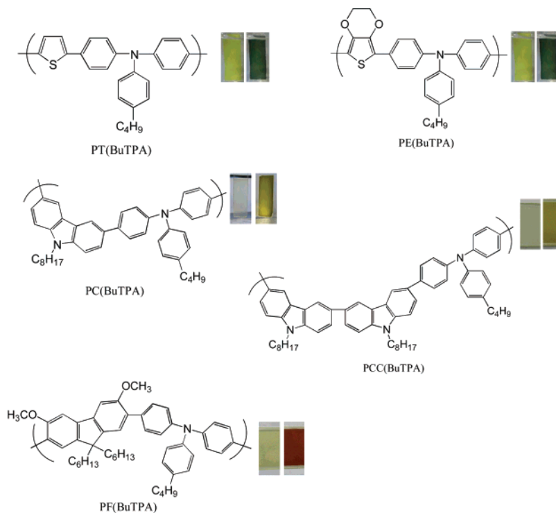
Scheme 2. Chemical Structure and Color Transitions of the Copolymers
